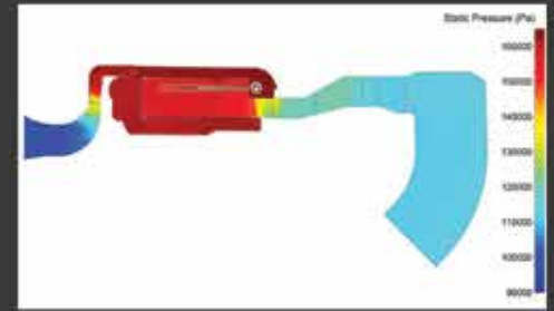
Meridional cutting plane colored by total pressure of KJ66 fully-coupled simulation
