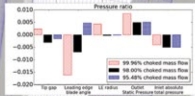
Sensitivity of solution with respect to uncertainties
